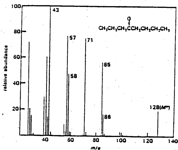
The mass spectrum of 4-octanone
