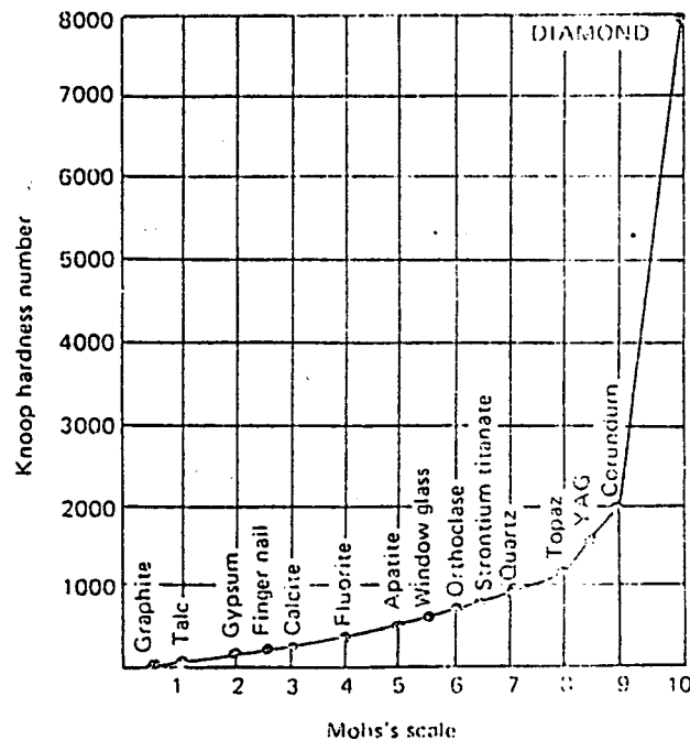
Figure 2.24. Diamond is the hardest substance known to man, natural or synthetic. The old Mohs's scale gives no idea of relative hardness, so it is here compared with an indentation hardness scale. (By courtesy of The Retail Jeweller)
