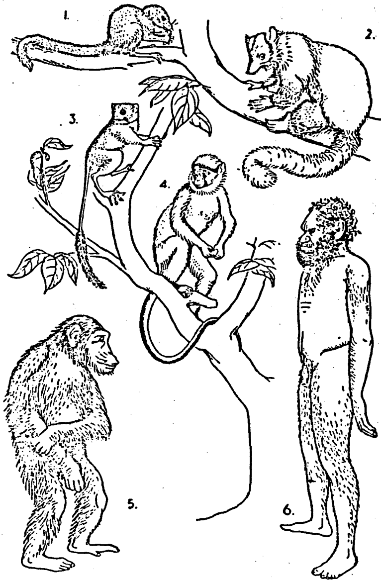
Figure 2. Some of the living members of the Order Primates, representing a gradational series which, broadly speaking, links man anatomically with some of the most primitive of placental mammals. (1) Tree-shrew; (2) Lemur; (3) Tarsier; (4) Cercopithecus monkey; (5) Chimpanzee; (6) Australian Aboriginal.
