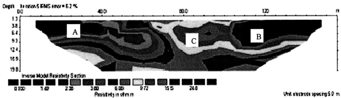
Fig. 8 Resistivity traverse 3, around Mundel Lake.
