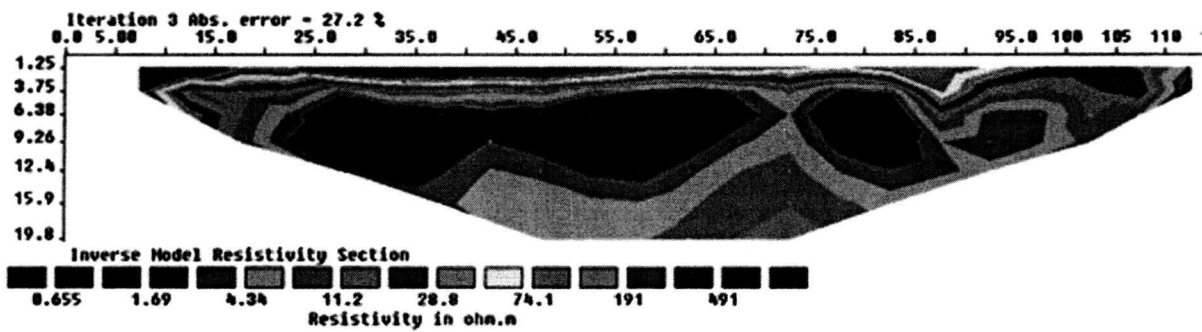
Fig. 10 Resistivity traverse around Rekawa lagoon area
