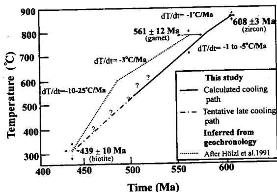
Figure 1. Calculated cooling paths of granulites from Sri Lanka from diffusion modelling (Fernando et al., 2003) compared with cooling rates inferred from geochronology (Hözl et al., 1991). The U-Pb zircon age of 608 \pm 3 Ma (Hözl et al., 1991) was assumed to represent the age of peak metamorphism in this diagram.
